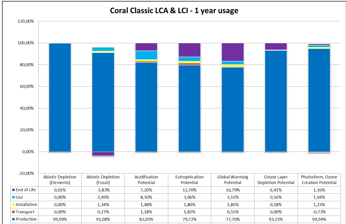
Figure 3: relative contribution of each process stage to each impact category for Coral Classic for a one year usage.
